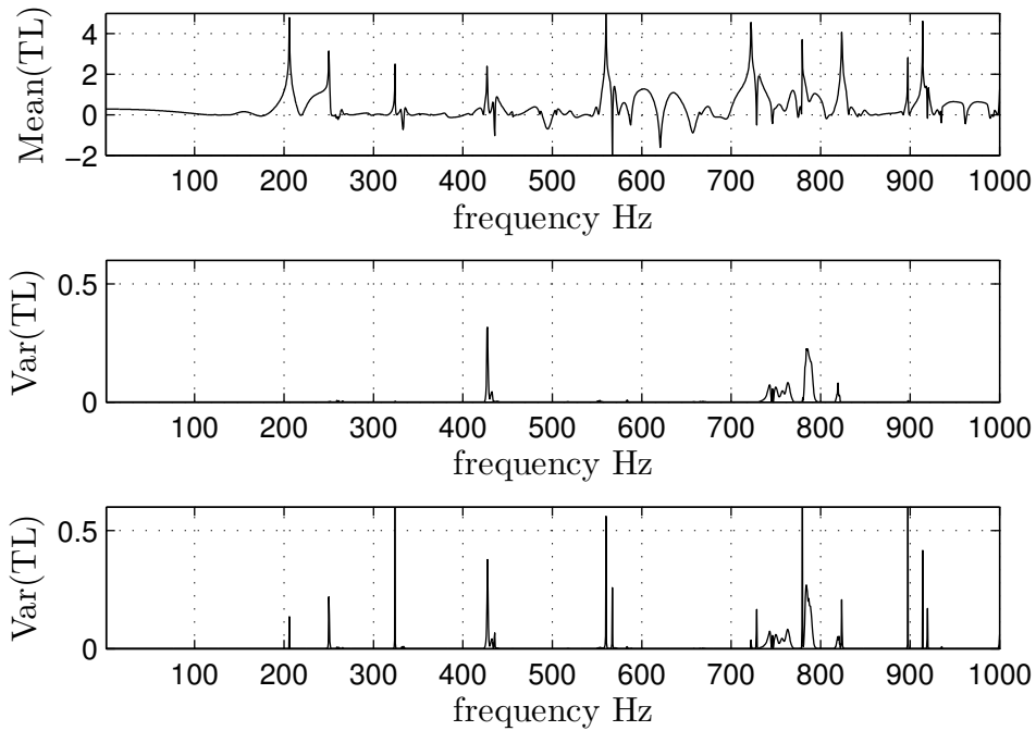
Figure 7: The mean of the TL (top). The variance of the TL when the slippage alone is randomized (middle) and both the slippage and the rigidities are randomized (bottom).
